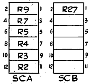
LAYOUT OF RESISTOR STRIPS
