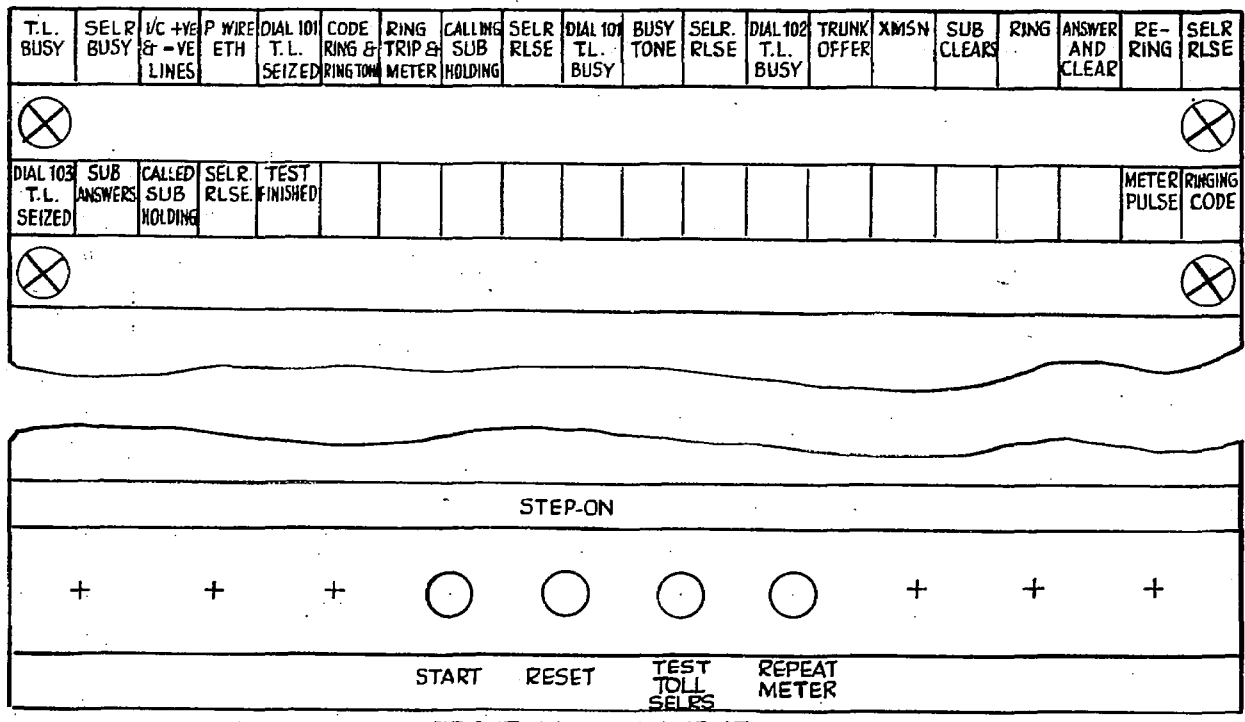
FRONT PANEL LAYOUT
