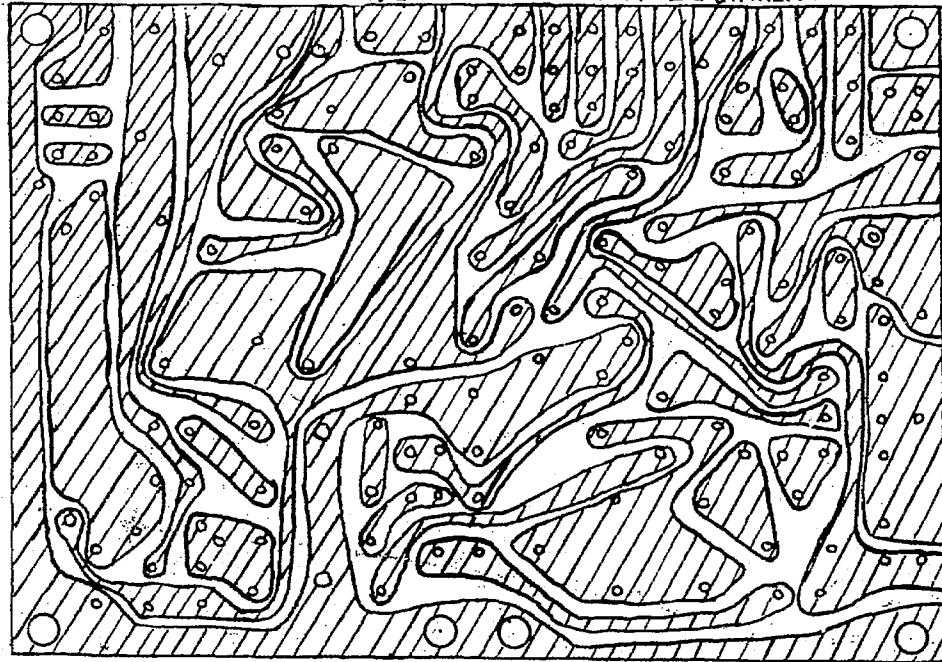
LAYOUT. PRINTED WIRING VIEWED FROM EQUIPMENT SIDE
