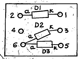
MTD. REAR OF LMA RELAY
