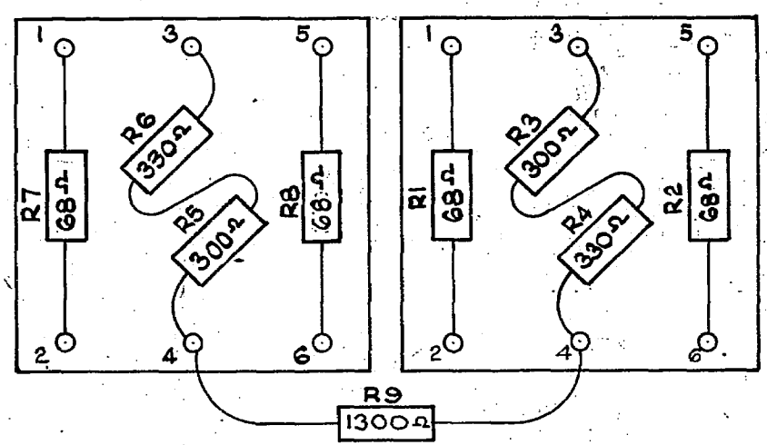
SCB LAYOUT
