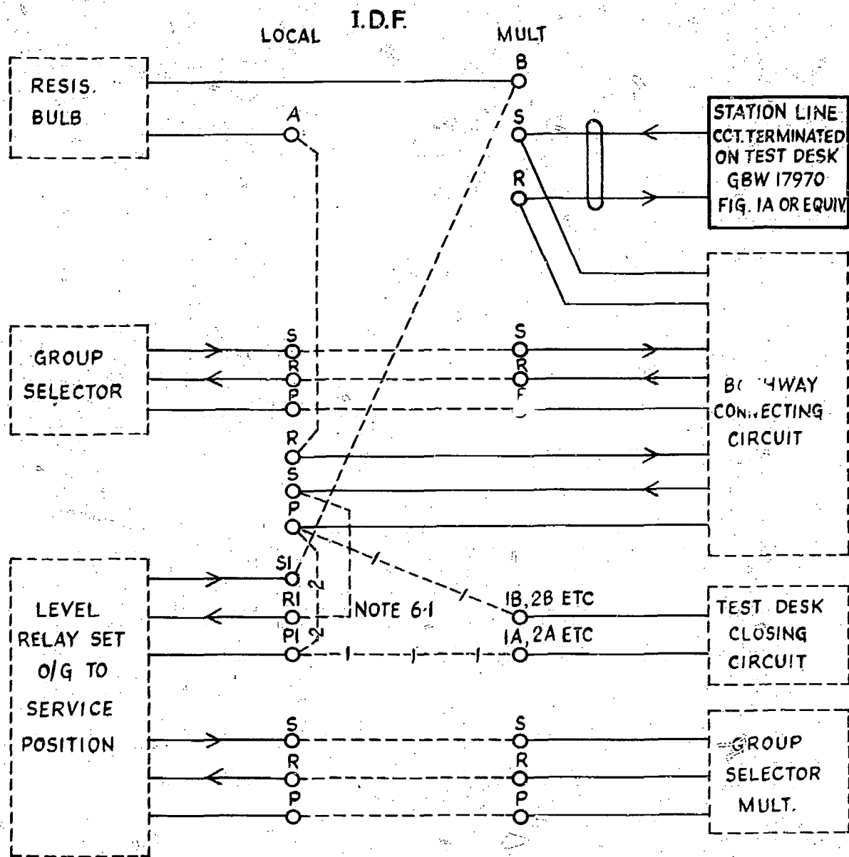
FIG. G B/W CIRCUIT (WHEN FIVE OR LESS TEST POSITIONS) VIA CONNECTING CIRCUIT
