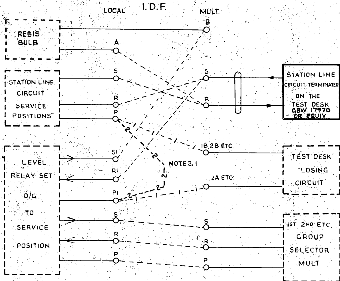
FIG. C B/W CIRCUIT (WHEN FIVE OR LESS TEST POSITIONS)
