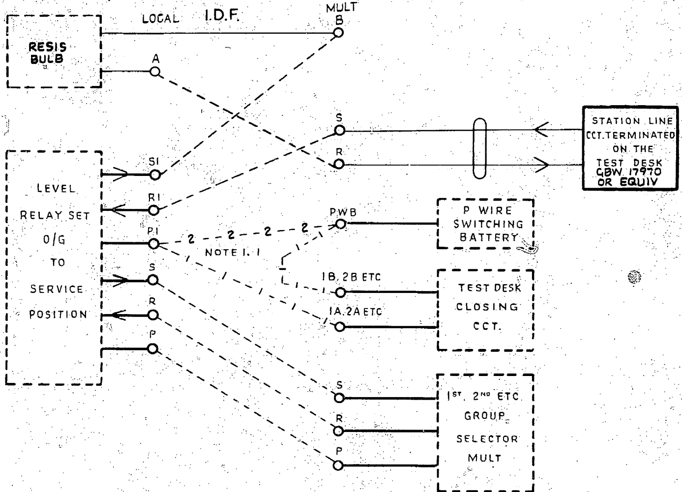
FIG B I/C ONLY CIRCUIT (WHEN FIVE OR LESS TEST POSITIONS)
