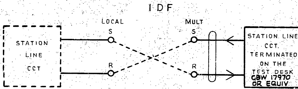
FIG A O/G ONLY CIRCUIT (WHEN FIVE OR LESS TEST POSITIONS)
