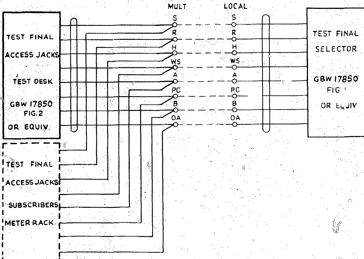
TYPICAL MARKING ON IDF
