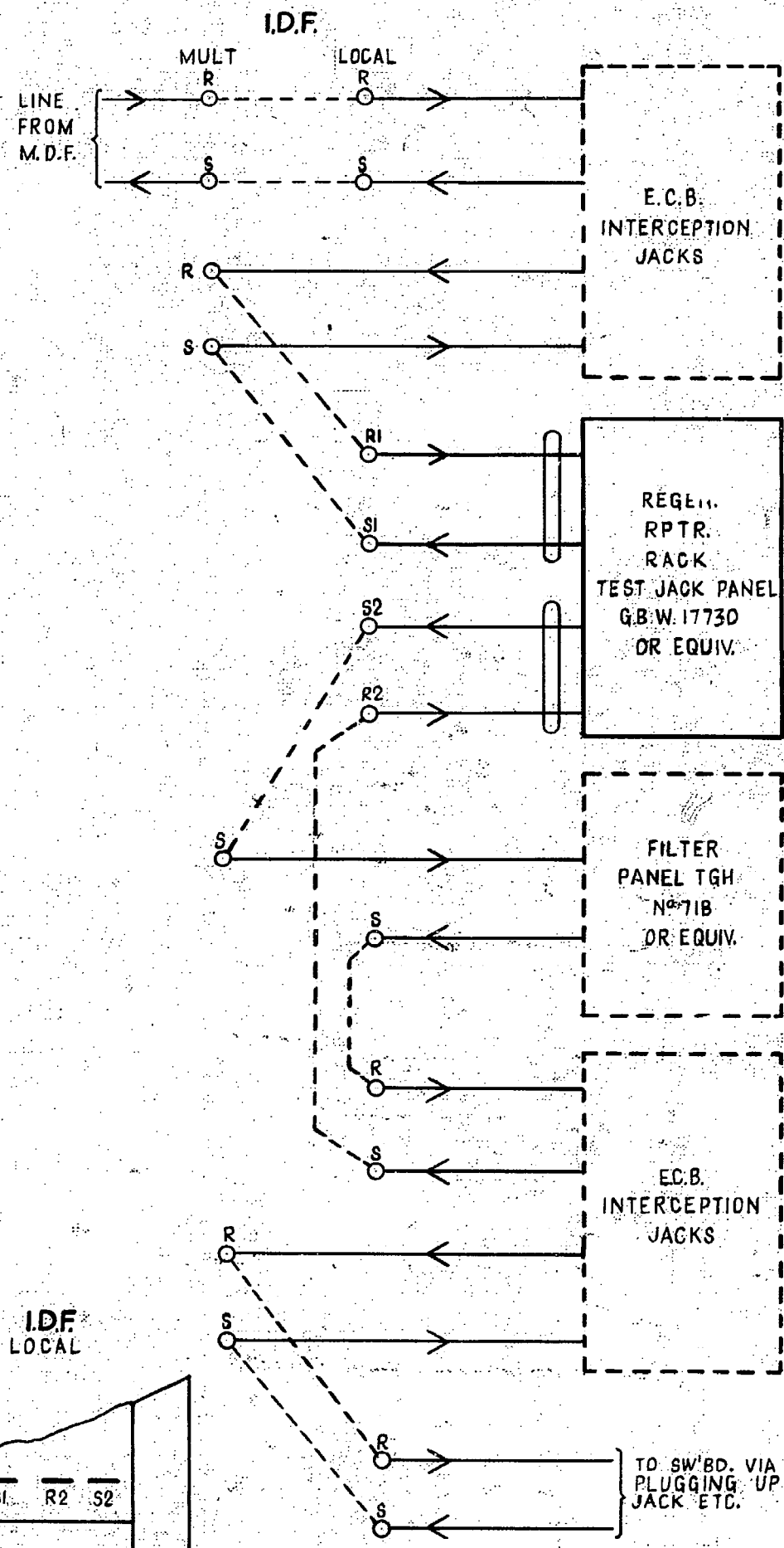
FIG. A JUMPERING OF REGENERATIVE REPEATER INTO RECEIVE LINE OF TELEX TRUNK CIRCUIT
