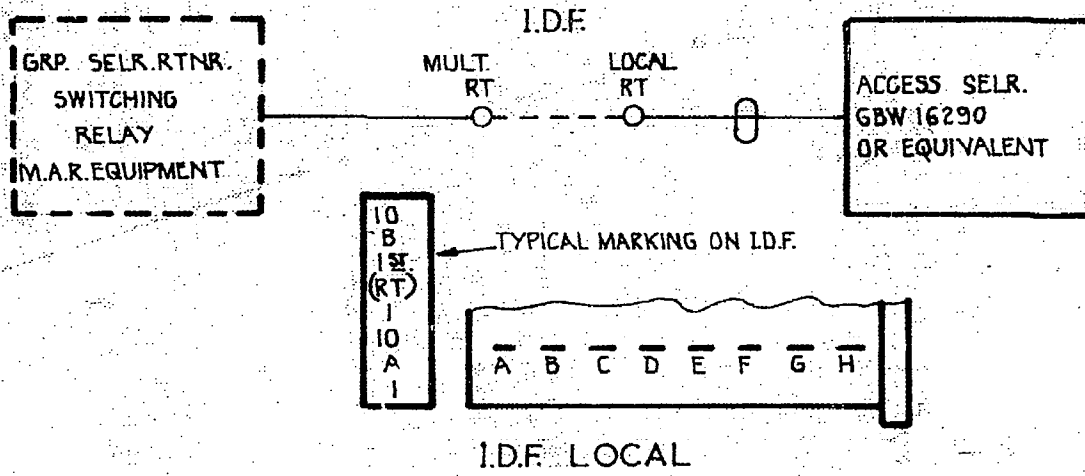
FIG. B T.D.F. TERMINATION FOR ACCESS SELRS. IN EXCHANGE WITHOUT I.D.F.
