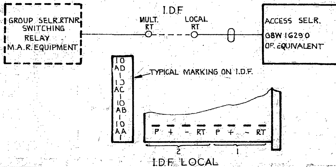
FIG. C I.D.F. TERMINATION FOR ACCESS SELRS. ASSOCIATED WITH GROUP SELRS. WITHOUT RACK GRADING FACILITIES.
