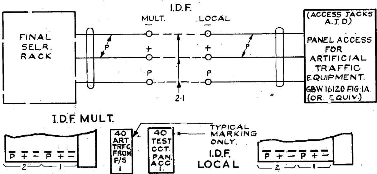
FIG. D. TEST NO. CIRCUIT NO. 1
