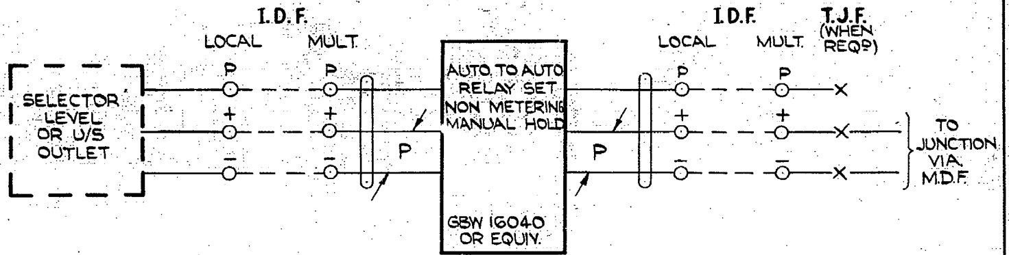
FIG. A INCOMING VIA I.D.F.
