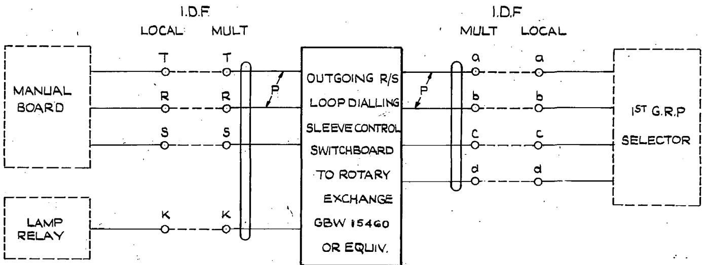
FIG. 1B. WHEN CABLED TO GROUP SELECTOR VIA I.D.F. MULT.
