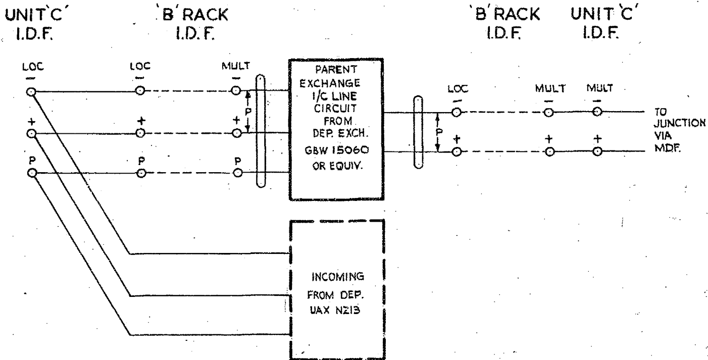
FIG. C. PARENT U.A.X. NZ 13. BOTHWAY WORKING.
