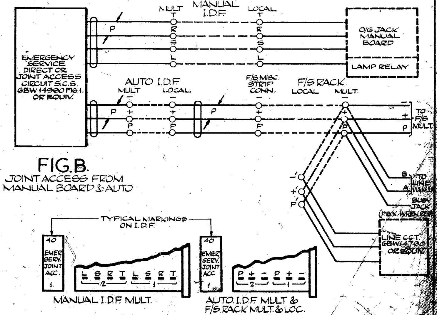
FIG. A. DIRECT ACCESS WITH I.D.F. CABLING BETWEEN R/S (UNI-DIRECTIONAL)
