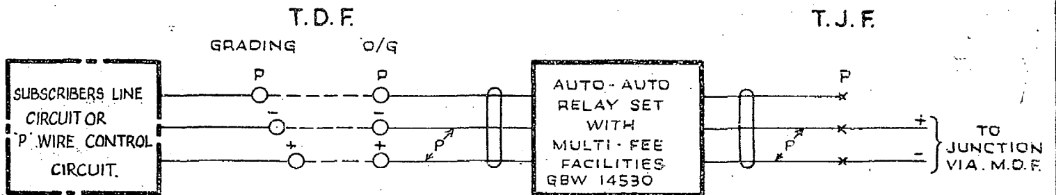
FIG. B CONNECTED VIA T.D.F.
