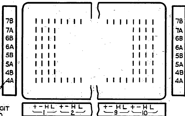
FIG. 1A. LEVELS SERVING 2ND SELRS., INT.-SW.BD. LINE CCTS., 'O' LEVEL CCTS. OR LAMP LIGHTING CCTS.
