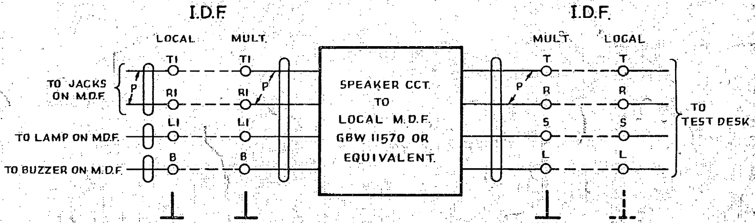
FIG. 2. TEST DESK CABLED VIA I.D.F.
