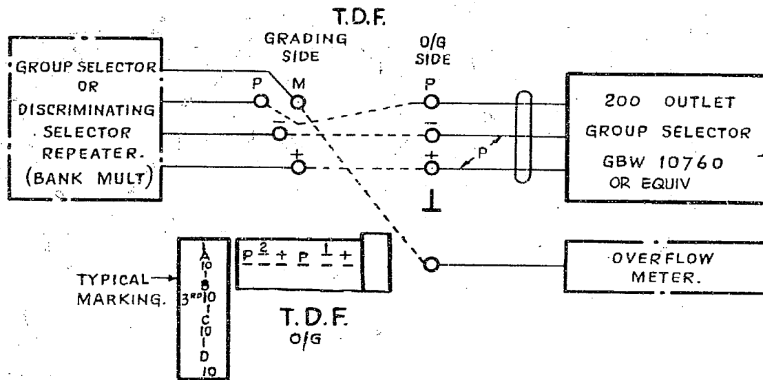
FIG. 2 200 OUTLET 1 ST GROUP SELECTOR CONNECTED VIA T.D.F.
