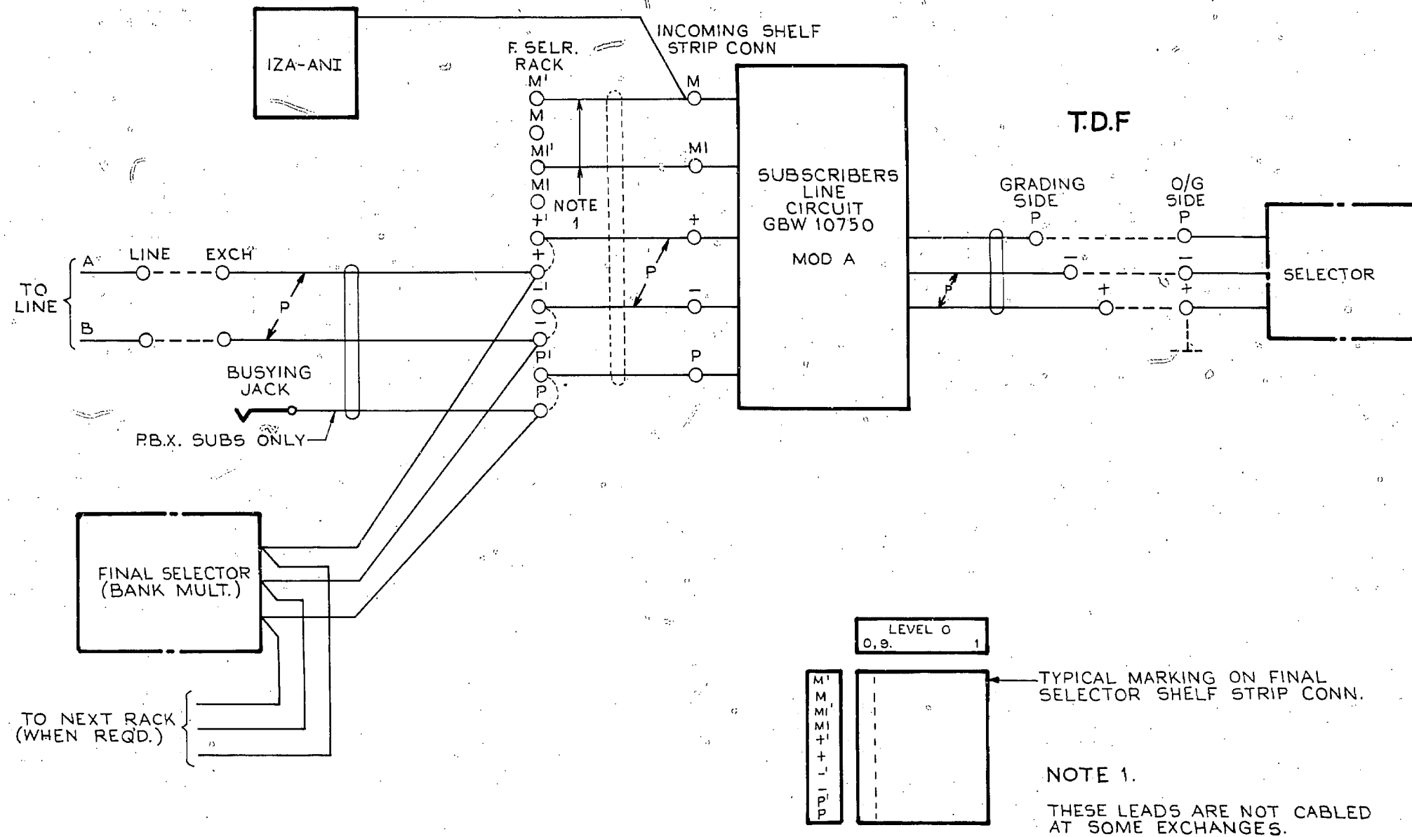
FIG. 1 REGULAR & 2-10 P.B.X. SUBSCRIBERS (WITH I.D.F. FACILITIES ON FINAL SELECTOR RACK.)
