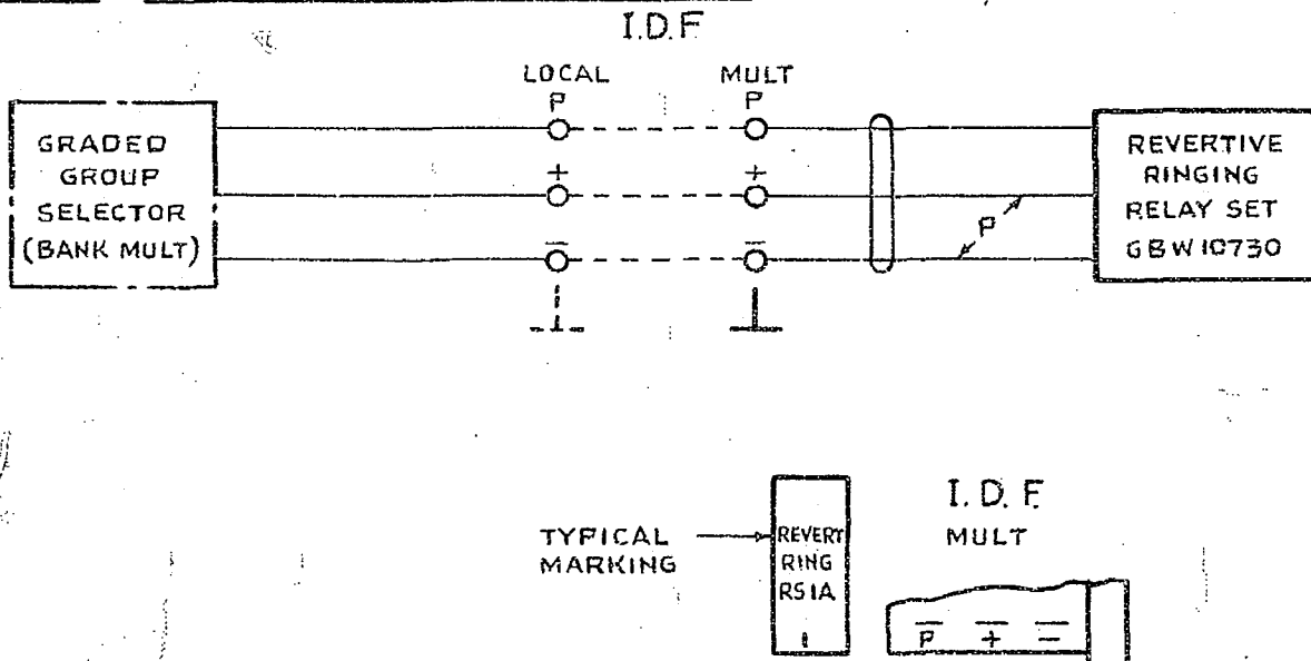
FIG. B CIRCUIT CONNECTED VIA I.D.F.
