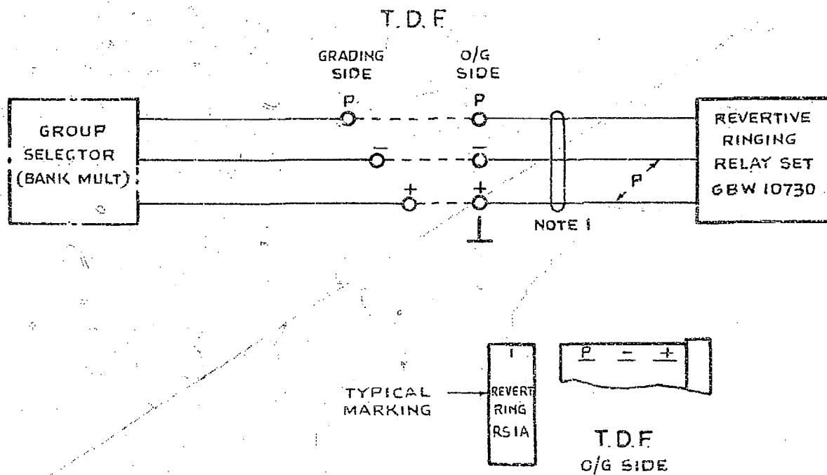
FIG. A CIRCUIT CONNECTED VIA T.D.F.
