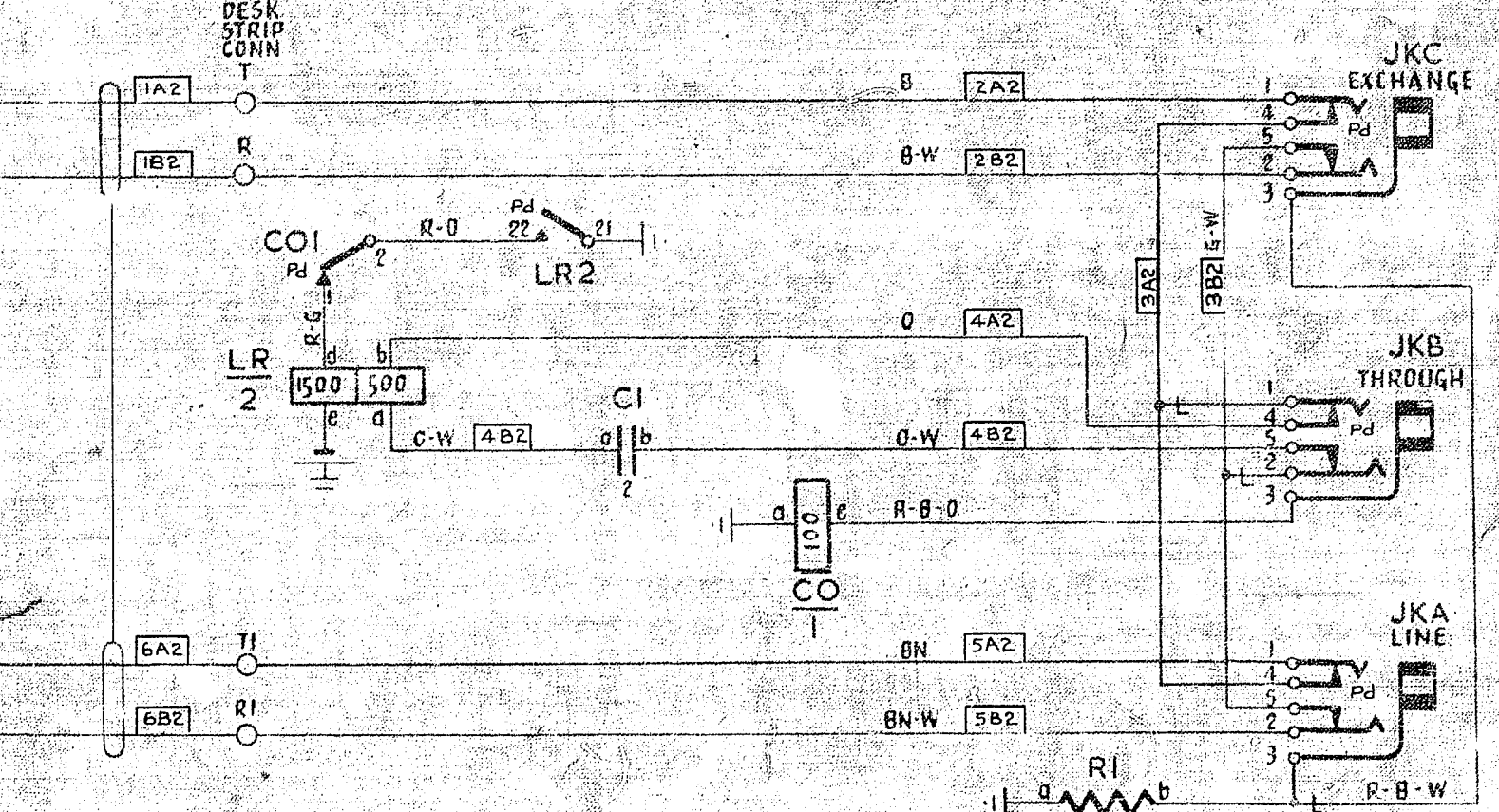
FIG. 2 TEST DESK
