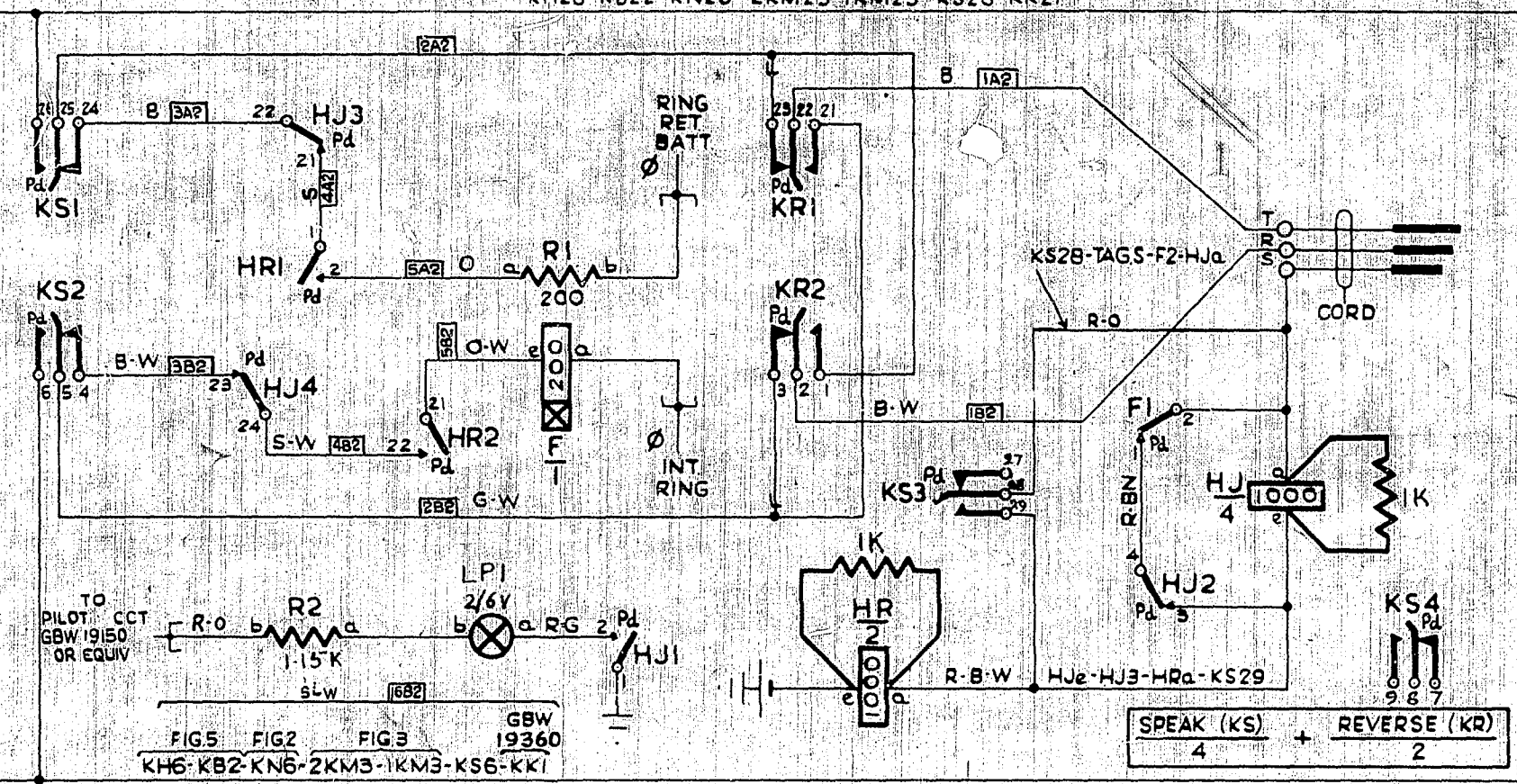
FIG. 1 RINGING CORD CIRCUIT
