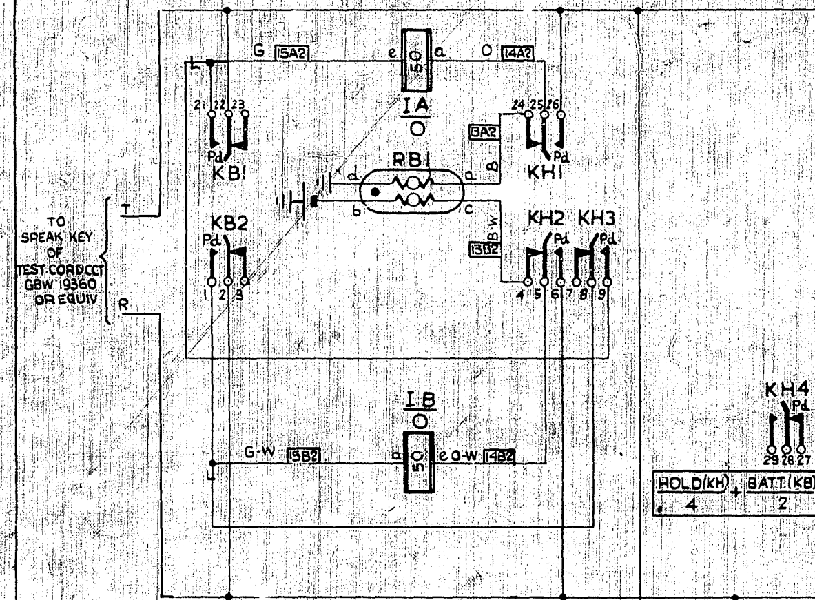
FIG. 5 BATTERY FEED CIRCUIT
