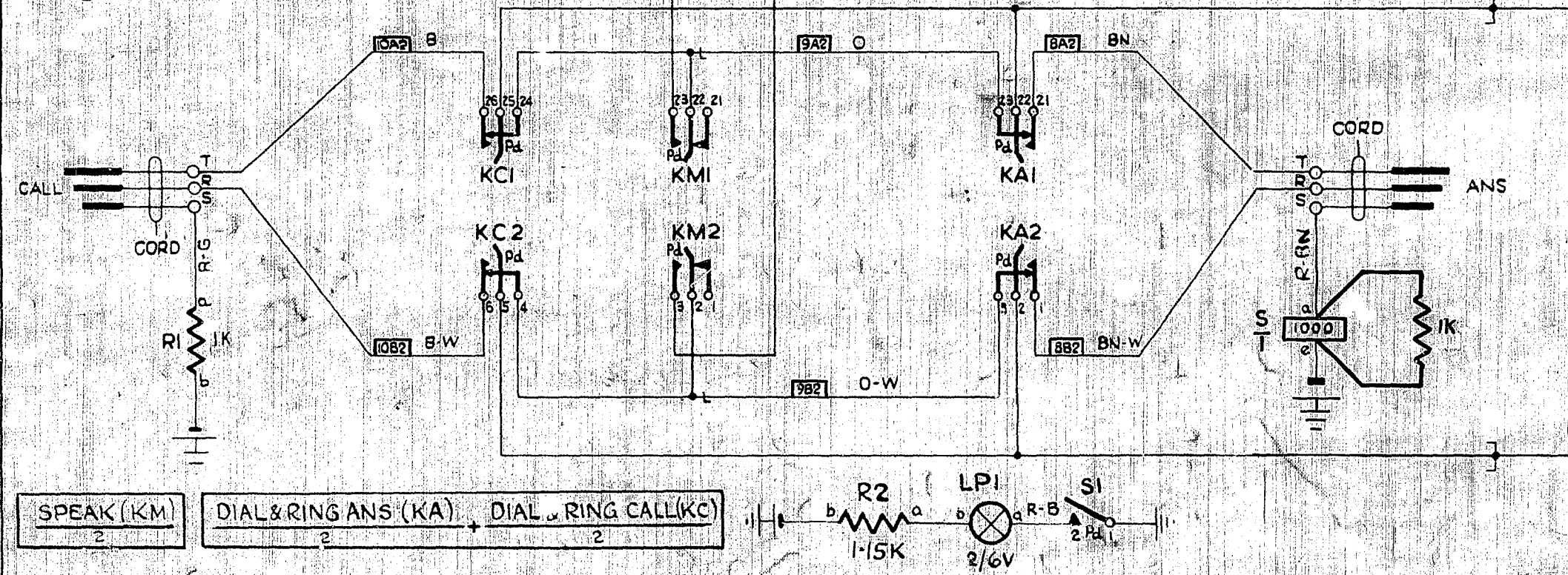
FIG. 3 CONNECTING CORD CIRCUIT
