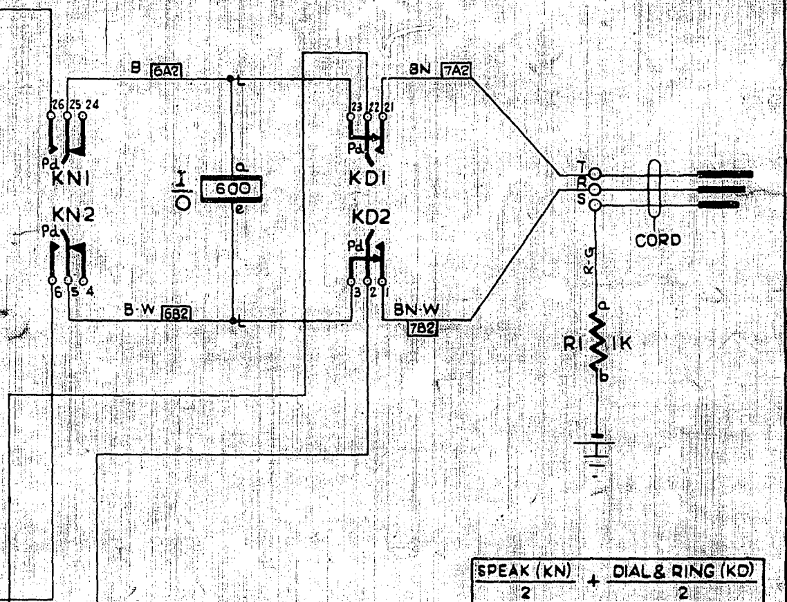
FIG. 2 SPEAKING CORD CIRCUIT
