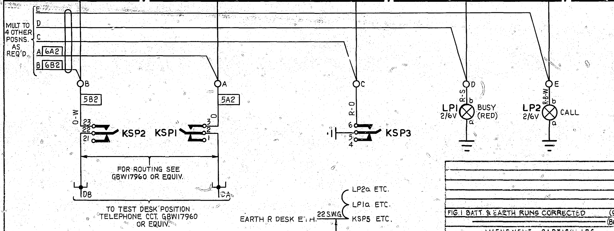
FIG.2 TEST DESK PER POSITION.
