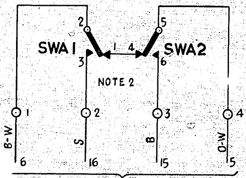
TO TEST JACK PANEL GBW 17730 OR EQUIV.
