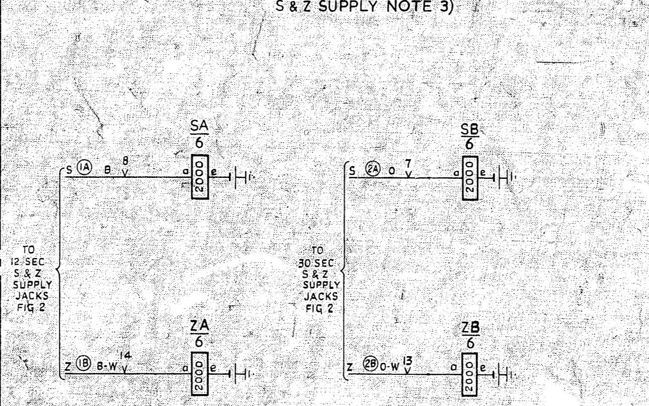
FIG 1 S & Z RELAY SET (1 ODD R/S & 1 EVEN R/S SERVE BOTH 12 SEC & 30 SEC S & Z SUPPLY NOTE 3)
