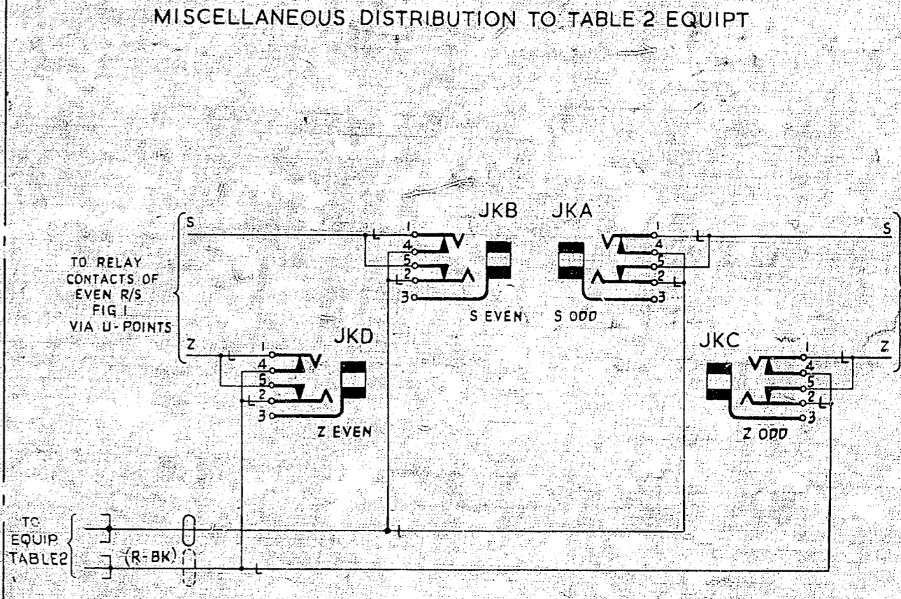
FIG 4 S & Z DISTRIBUTION (12 SECS OR 30 SECS) MISCELLANEOUS DISTRIBUTION TO TABLE 2 EQUIPT
