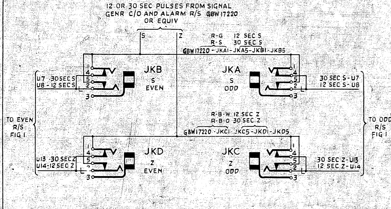
FIG 3 S & Z DISTRIBUTION TO RACKS (12 OR 30 SECS) TABLE 1 EQUIPT
