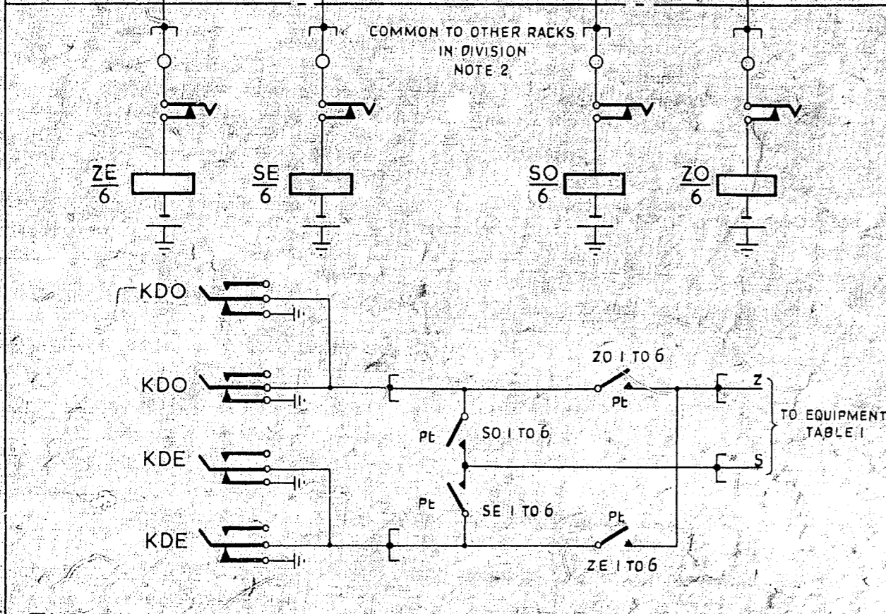
FIG 5 RACK DISTRIBUTION EXPLANATORY ONLY
