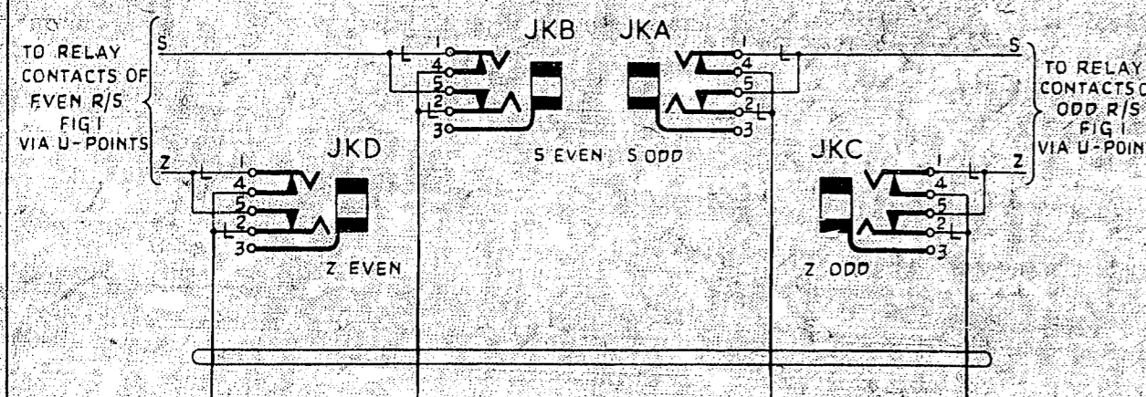
FIG 3 S & Z DISTRIBUTION TO RACKS (12 OR 30 SECS) TABLE 1 EQUIPT
