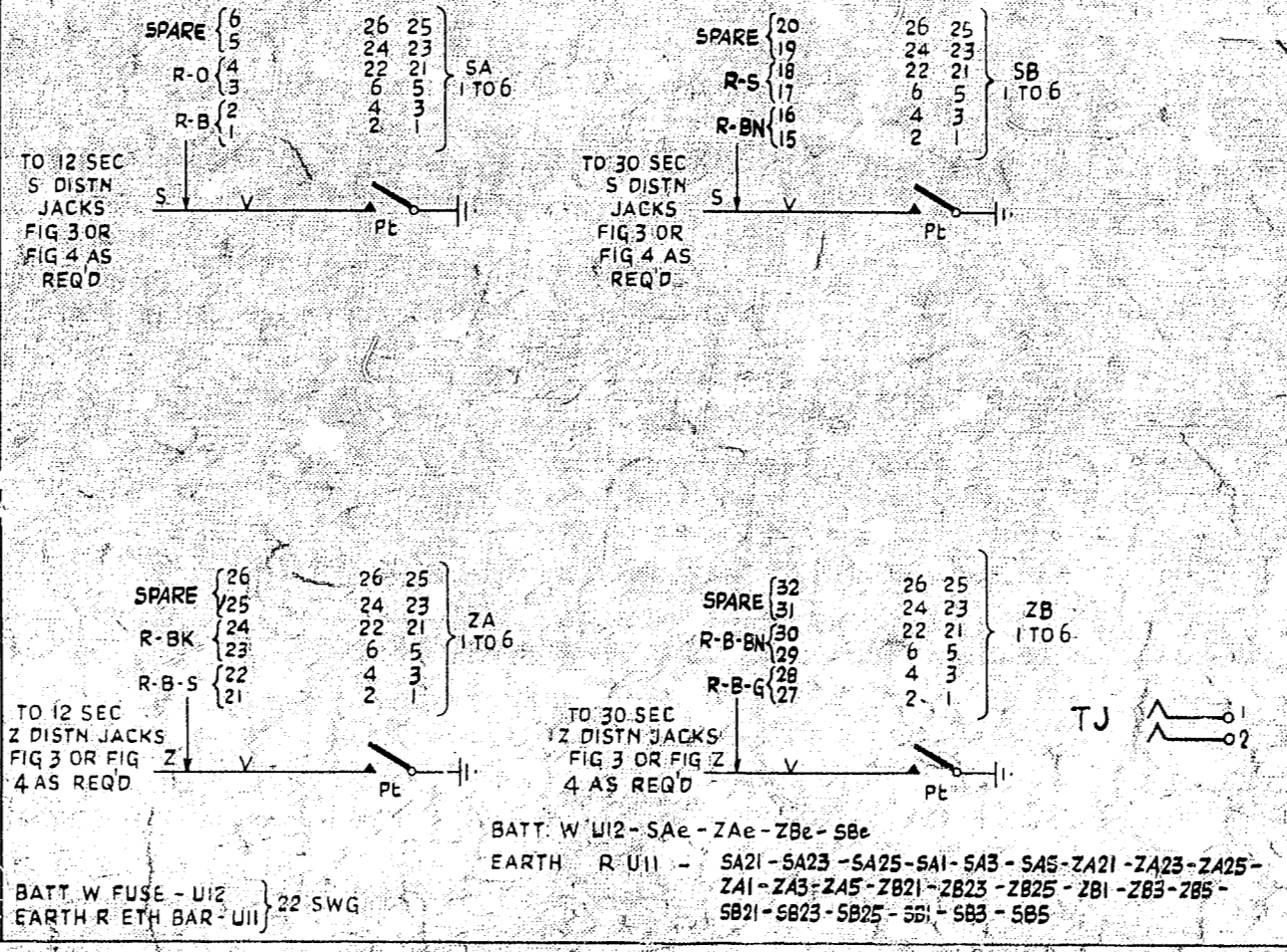
FIG 5 RACK DISTRIBUTION EXPLANATORY ONLY
