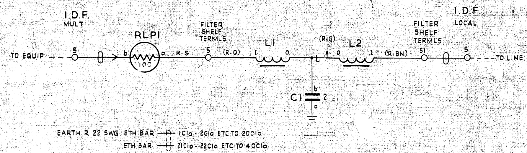
FIG. 1 LINE FILTER CIRCUIT M.A.R.
