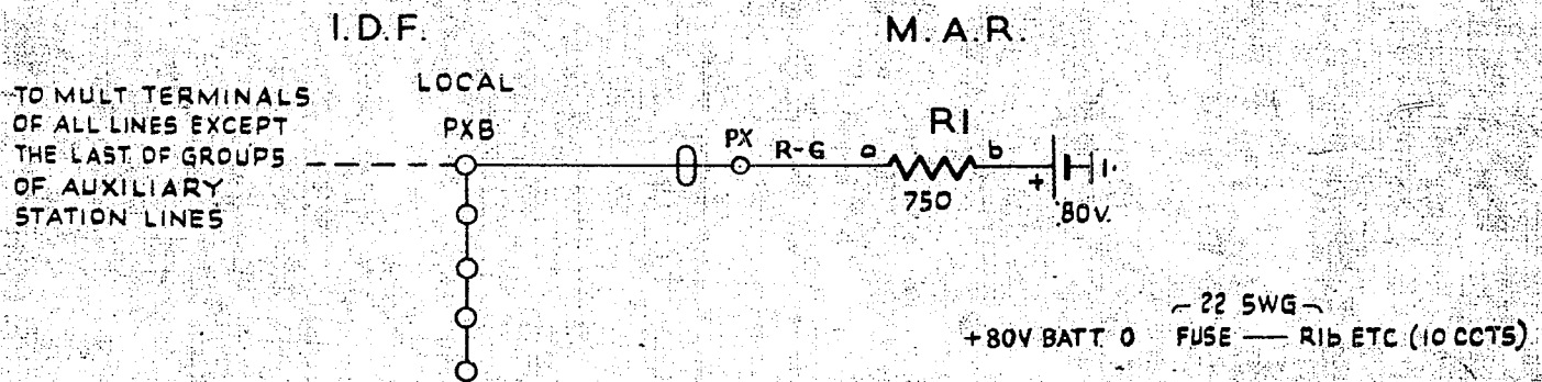
FIG 2 HUNTING BATTERY (PX) FOR GROUPS OF AUXILIARY STATION LINES
