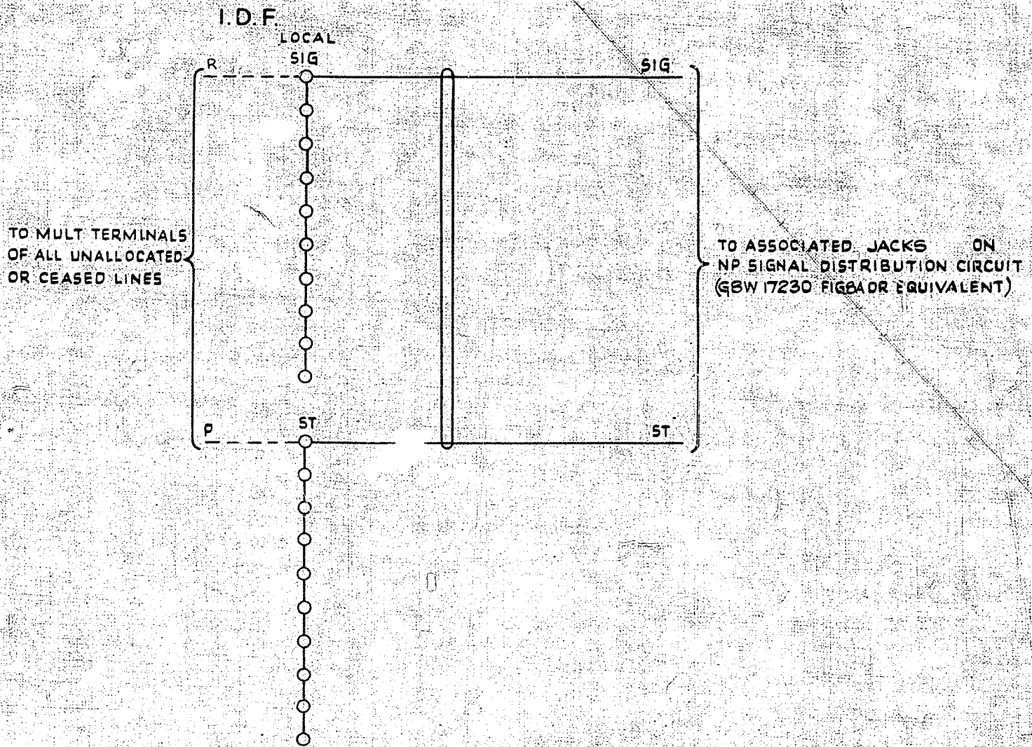
FIG 1 NP FOR SPARE LINES
