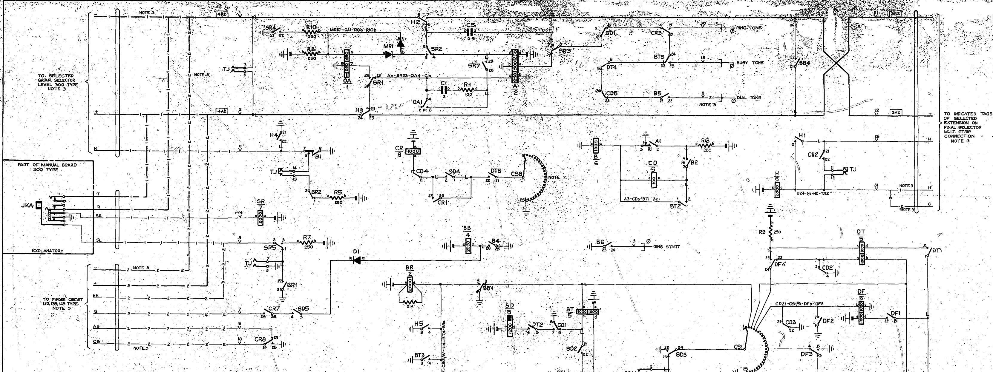
FIG. 2 AUDIBLE CODE CALL AUXILIARY CIRCUIT.
