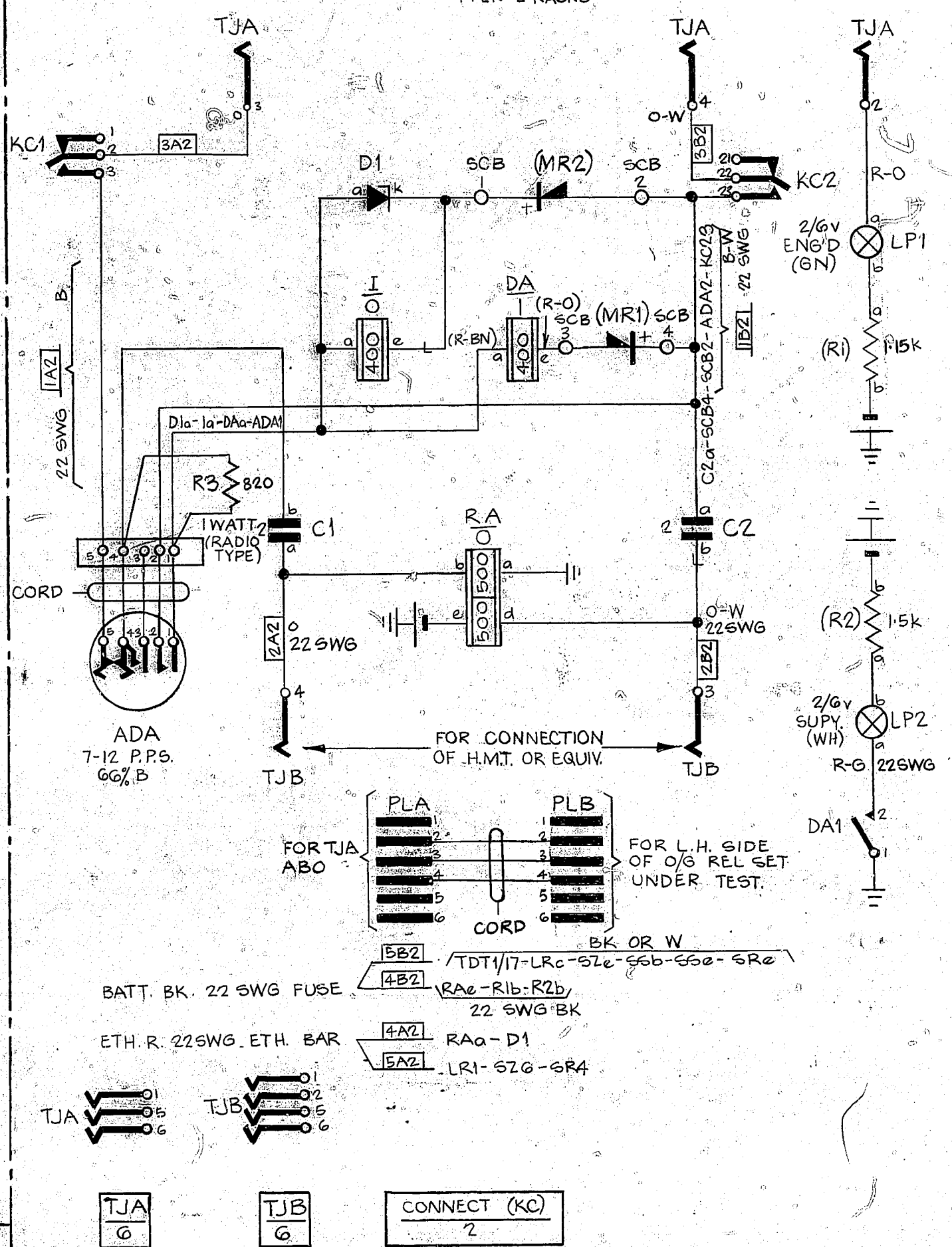
FIG. 2 TEST CIRCUIT
