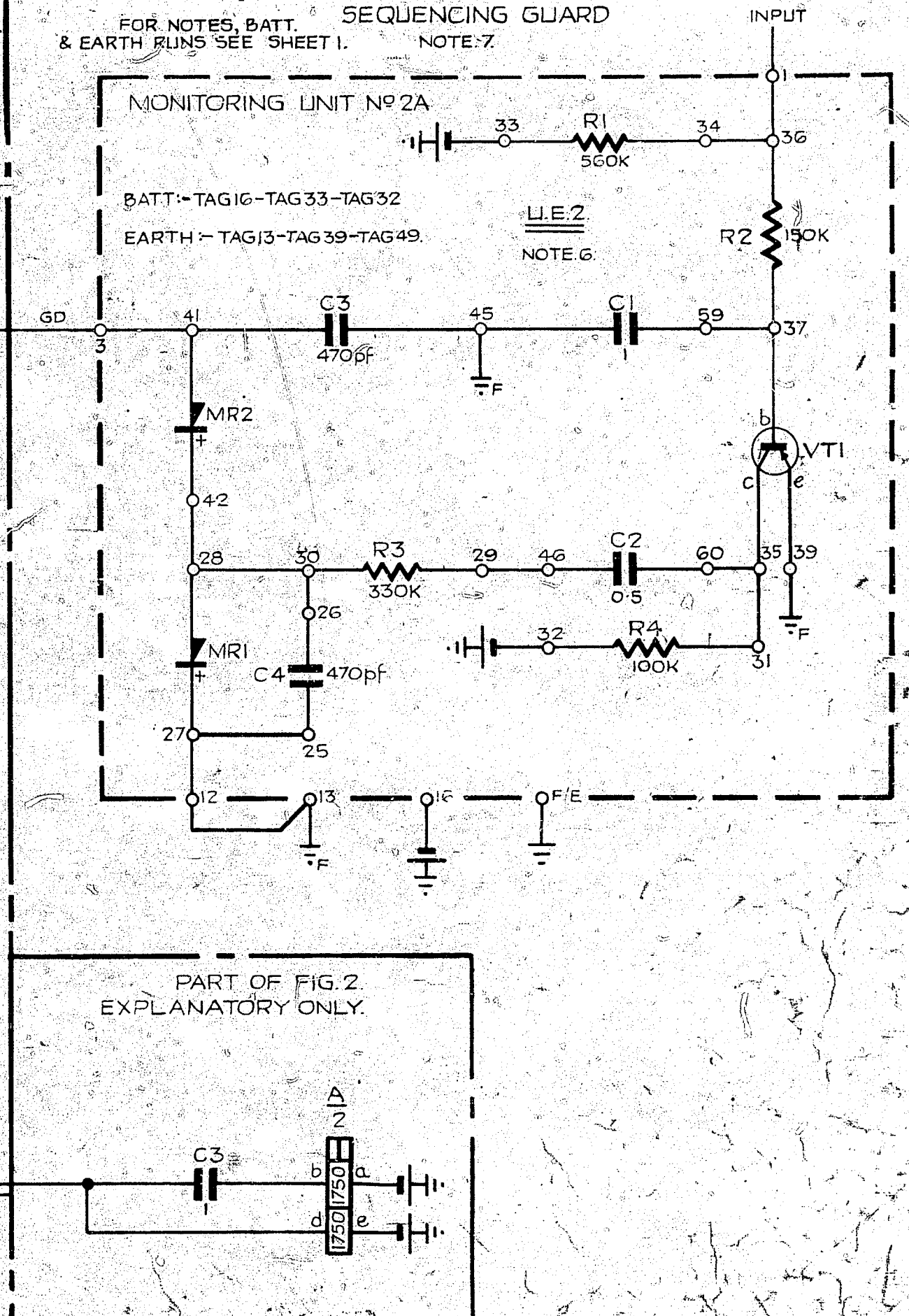
FIG. 6. SEQUENCING GUARD
