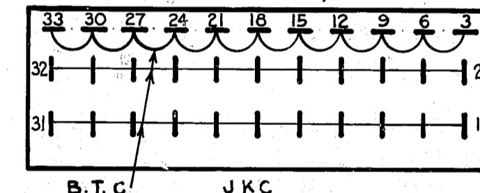
FIG. ID. REMOTE ANSWERING PLUG (FOR USE WITH JACK AJC)
