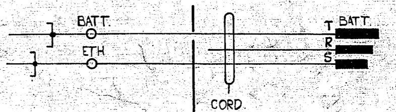
FIG.3. BATTERY PLUG
