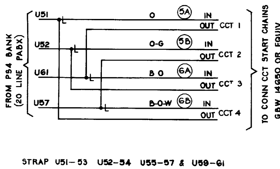
FIG 1B CONN CCT START CHAIN
