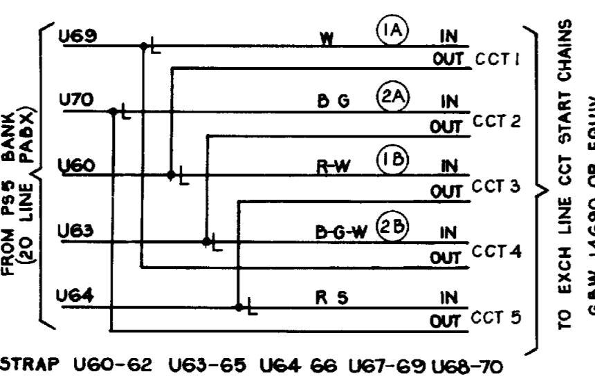
FIG 1C EXCH LINE CCT START CHAIN
