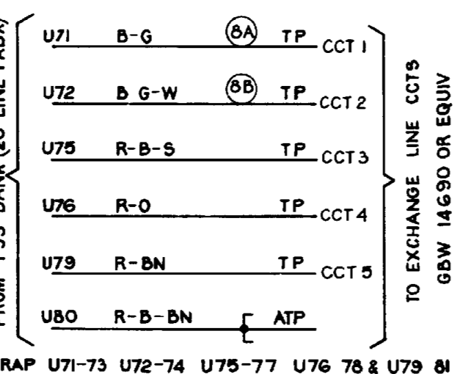
FIG 1D TEST PULSES
