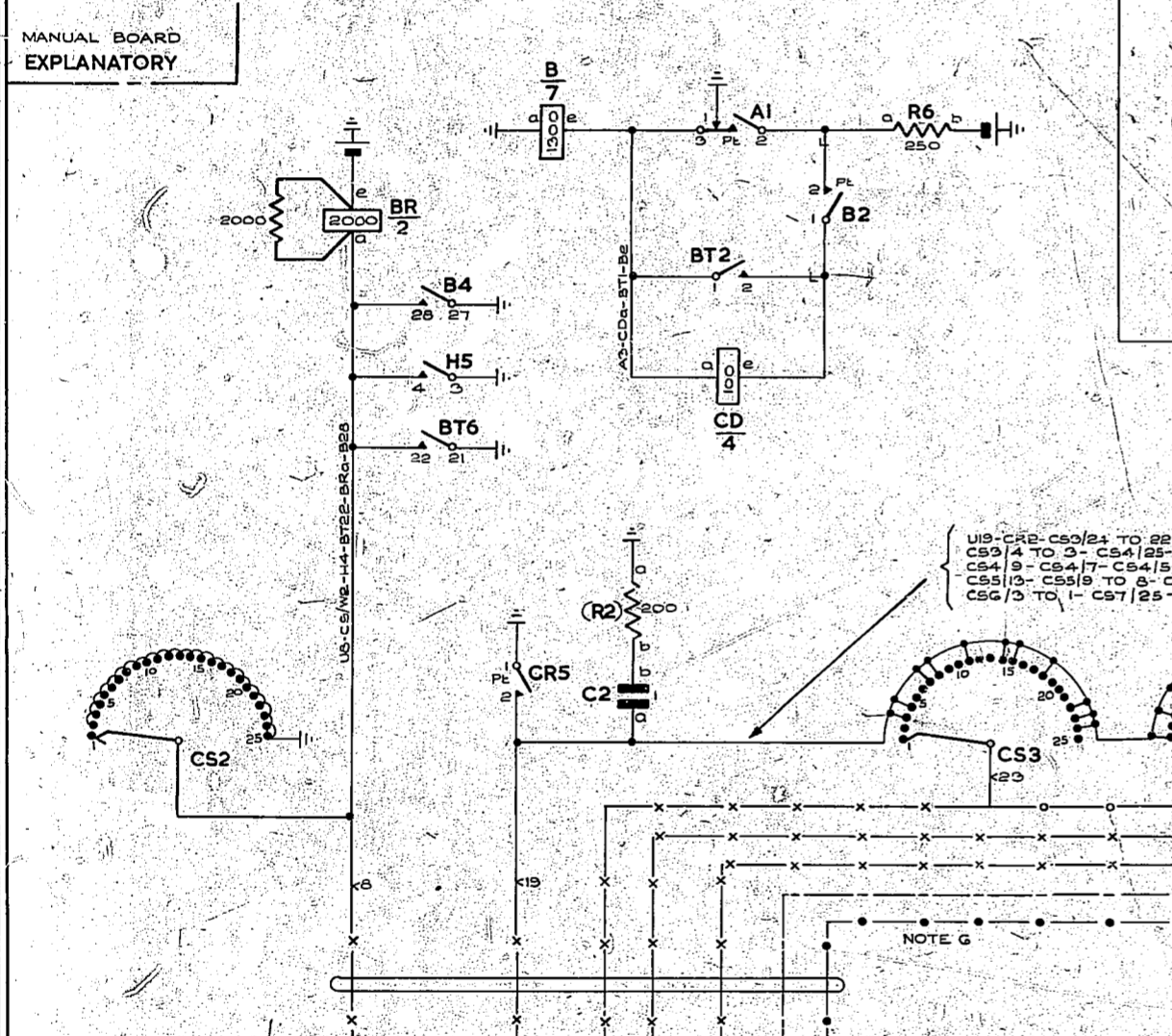
FIG. 2. AUDIBLE CODE CALL AUXILIARY CIRCUIT.
