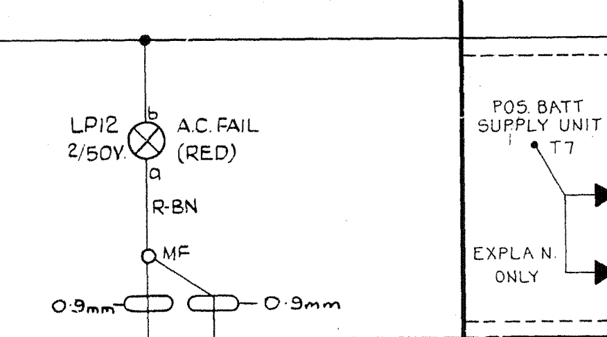
FIG.33 50V. POSITIVE SUPPLY FAIL ALARM 1 PER GRP. OF UNITS 'S'
