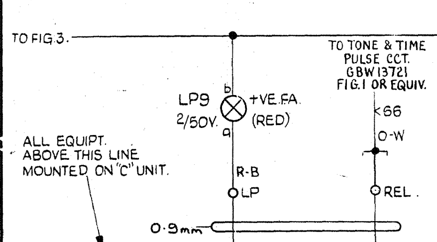
FIG.30 FUSE ALARM POSITIVE BATTERY SUPPLY 1 PER GRP. OF UNITS 'S'
