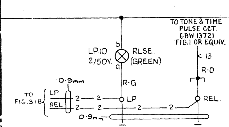
FIG.31 RELEASE FAILURE ALARM (10 SECS. APPROX.) 1 PER GRP. OF UNITS 'S'
