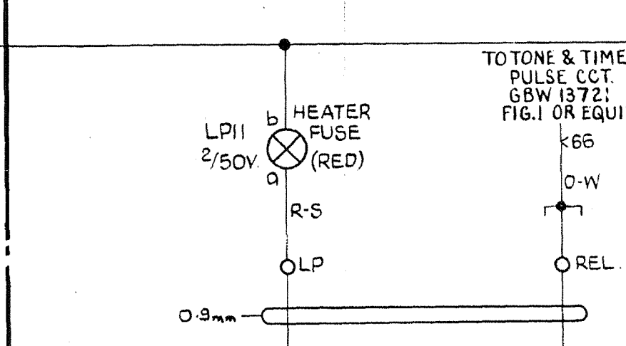
FIG.32 FUSE ALARM HEATER SUPPLY (I.V.F.) 1 PER GRP. OF UNITS 'S'
