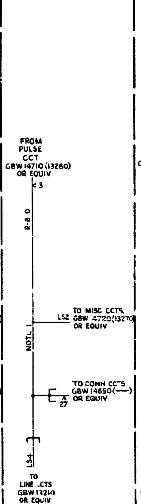
FIG 4 LINE START 1 PER P A B X
