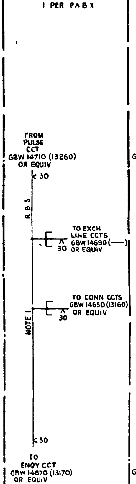
FIG 8 RING TONE DISTRIBUTION 1 PER P A B X
