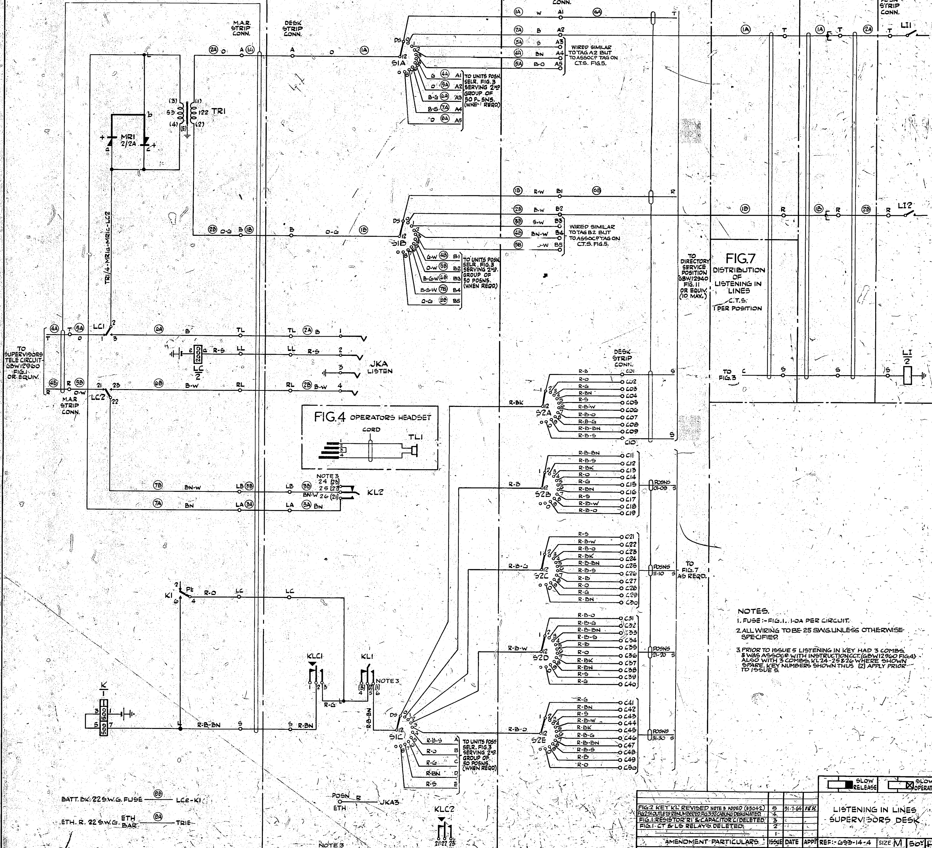
LISTENING IN CIRCUIT ON MANUAL BOARD PART OF GBW2910 OR EQUIV. EXPLANATORY ONLY POSN STRIP CONN.
