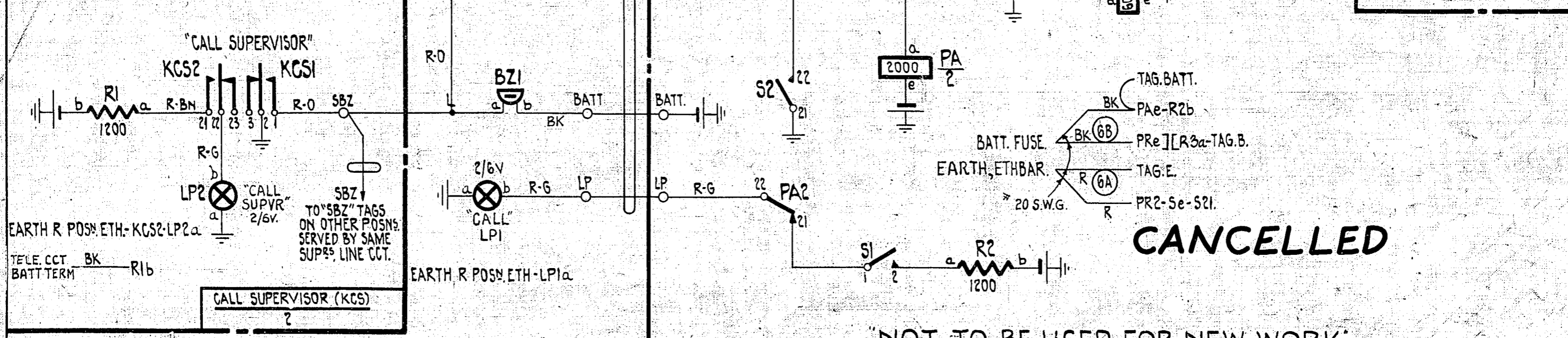
FIG.2 CALL SUPERVISOR C'CT.
