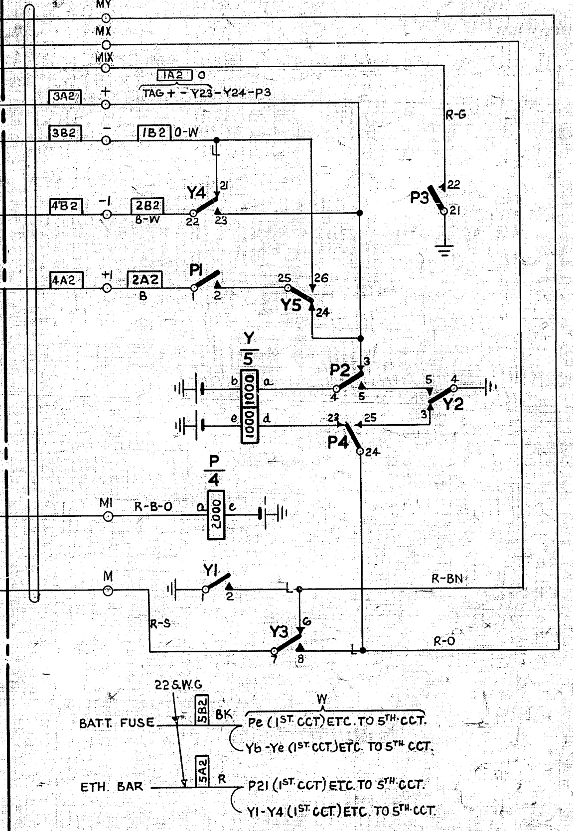
FIG. 2 METER DISCRIMINATION RELAYS (M.A.R.)
