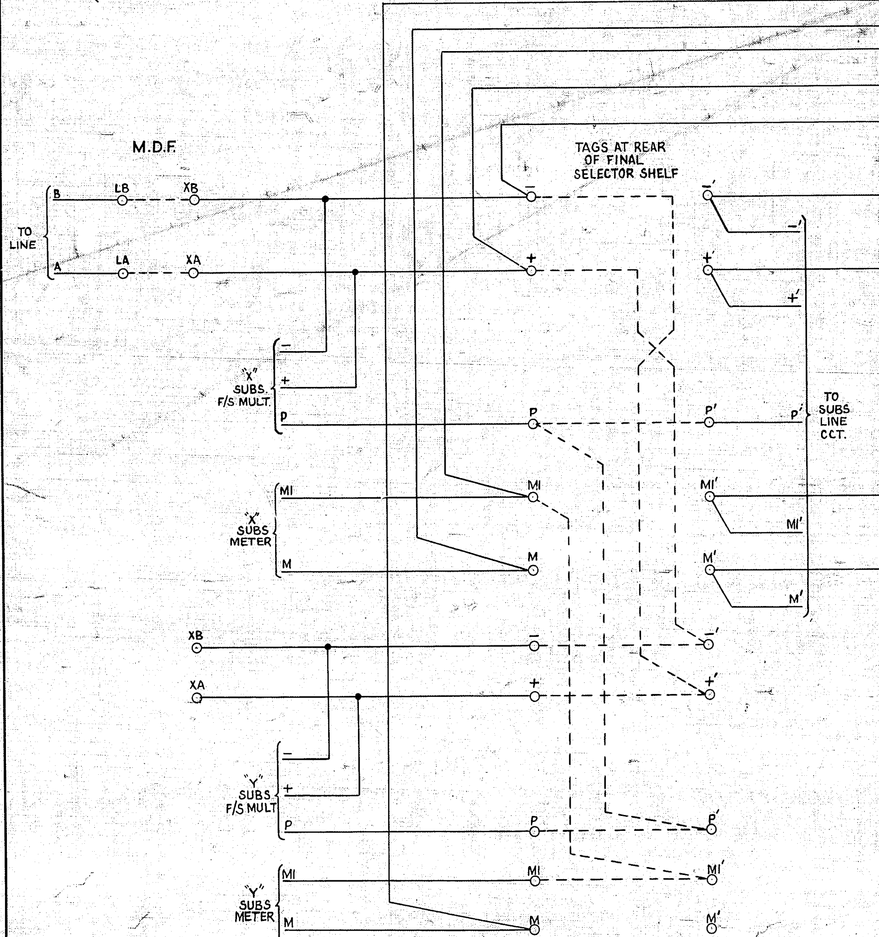
FIG. 1 PART OF SUBS LINE CCT (NOTE 3) (EXPLANATORY ONLY)
