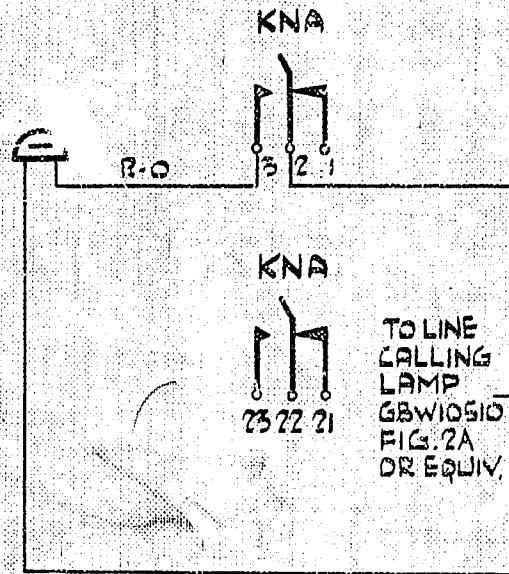
FIG.1 TEST JACK FRAME OR O.G.J. BUSYING PANEL T.J.F.
