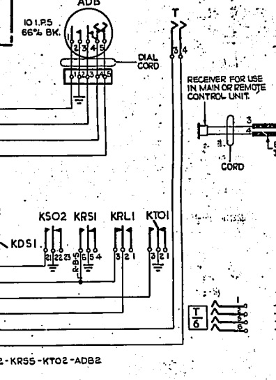
FIG. 2. REMOTE CONTROL UNIT.
