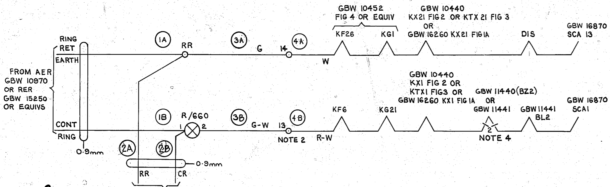
FIG 2. CONT RINGING TO ALTERNATE DESKS.
