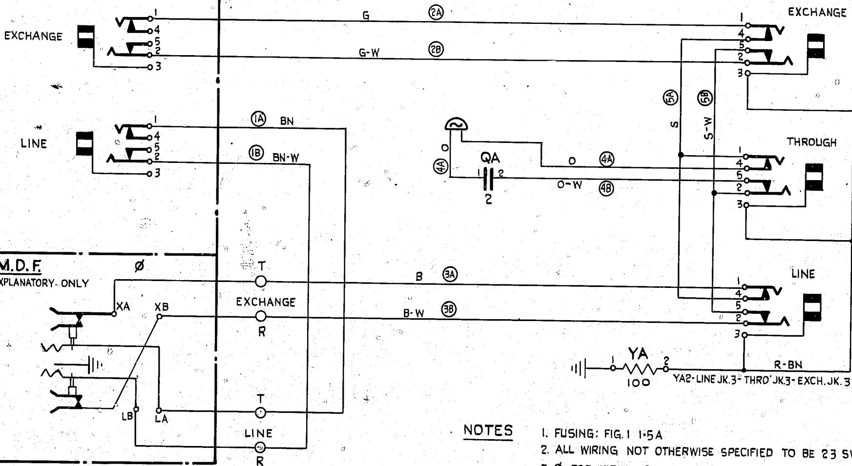
FIG 2A TEST RACK
