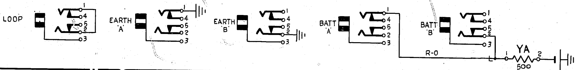
FIG 2B TEST JACK FIELD
