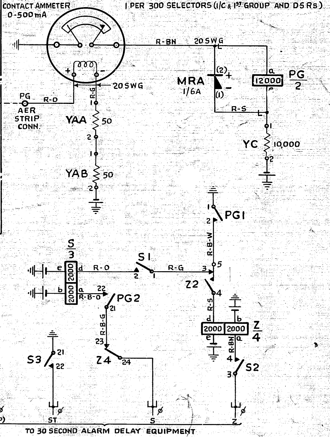
FIG. 2 ALARM EQUIPMENT A.E.R.
