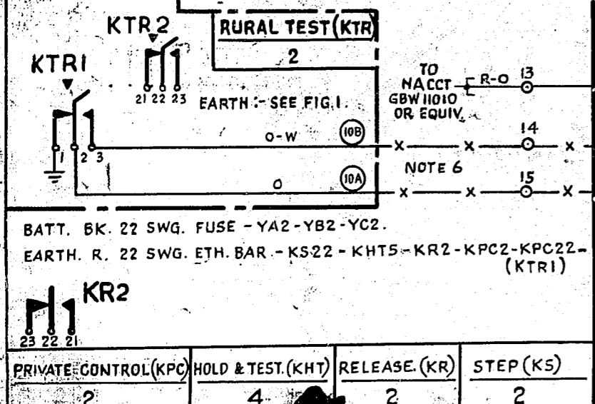
FIG.3 RURAL LINE TEST CCT. 1 PER TEST SELECTOR WHEN SPEC'D. NOTE 6.
