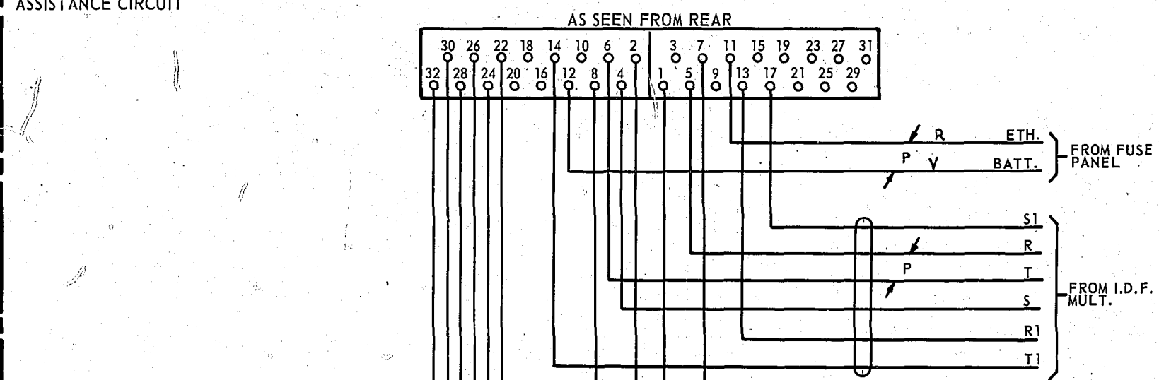
FIG.2. ASSISTANCE CIRCUIT
