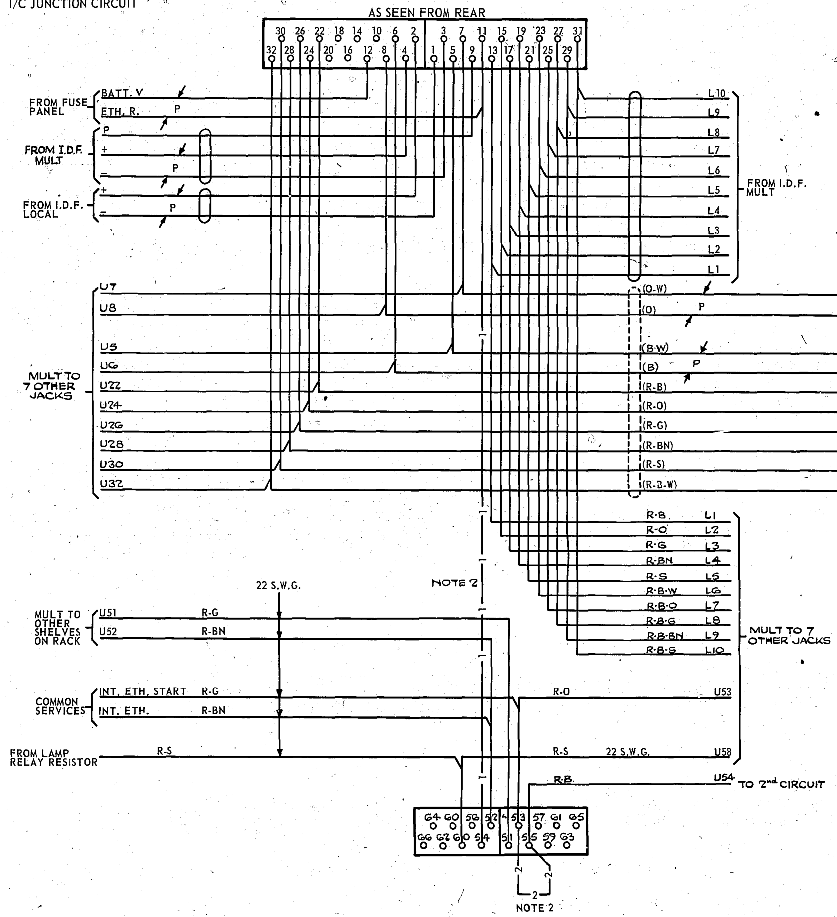
FIG.1. I/C JUNCTION CIRCUIT
