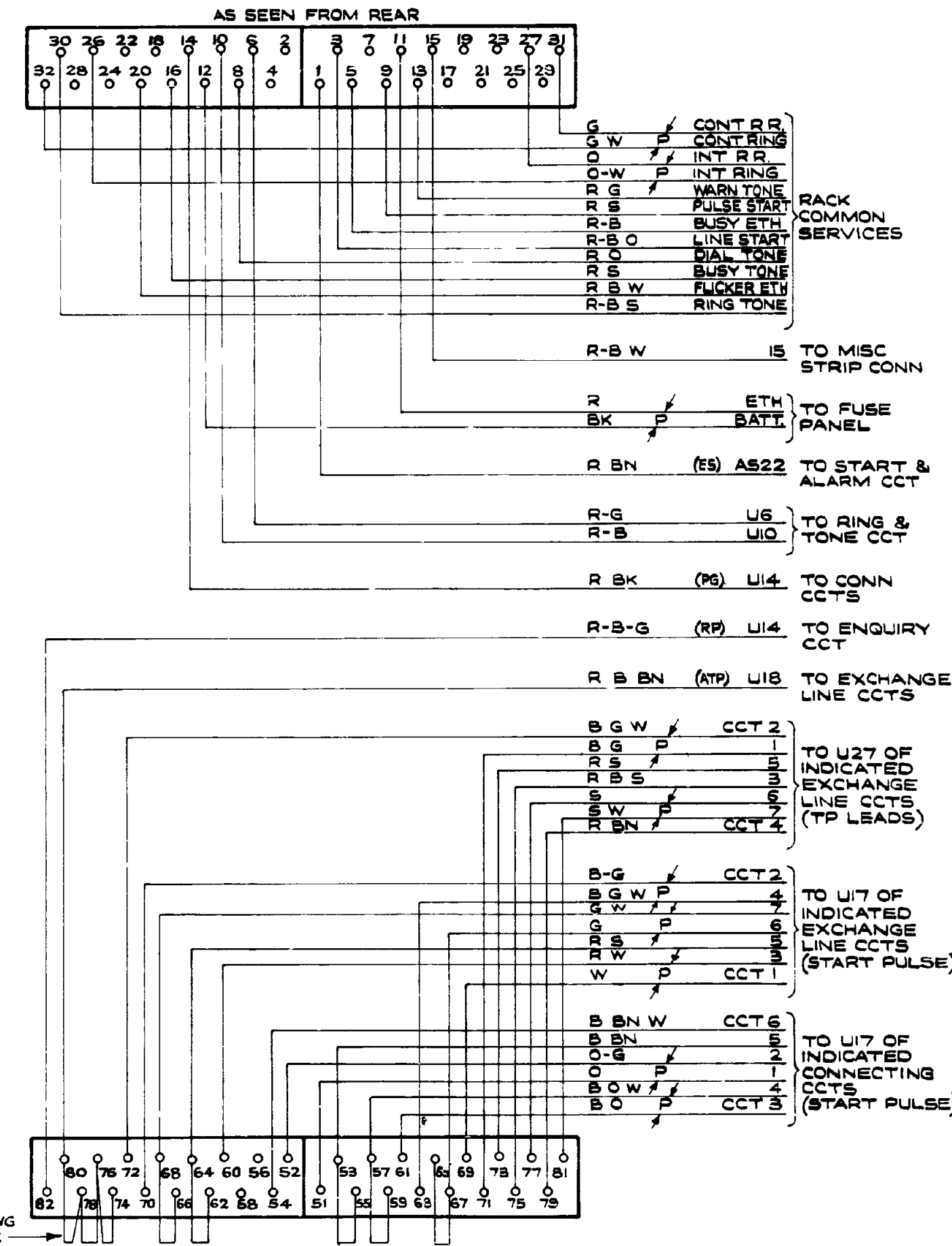
FIG. 1B. 35-LINE PABX
