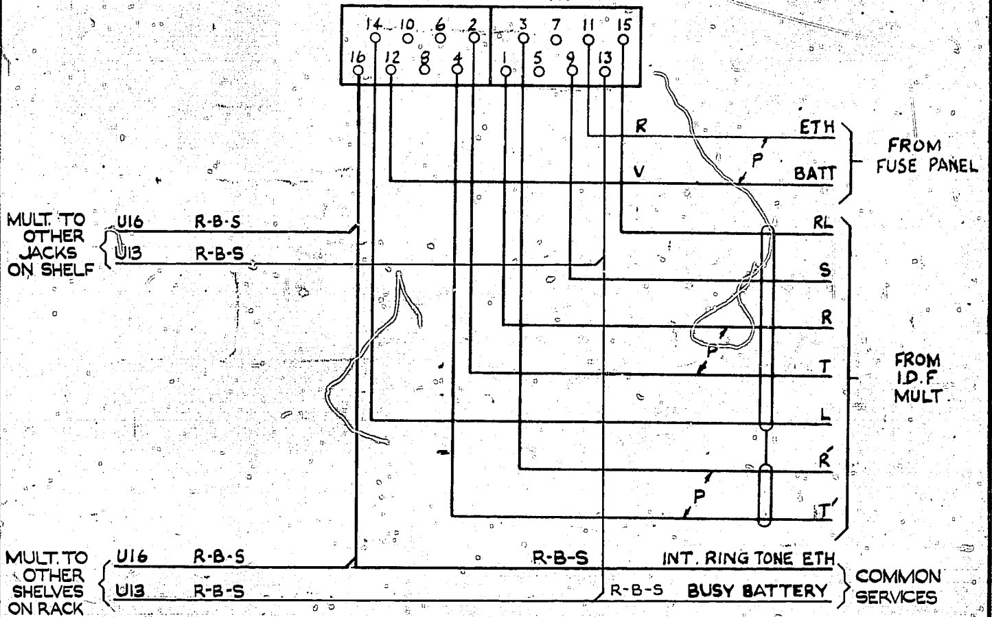
FIG.1 AS SEEN FROM REAR
